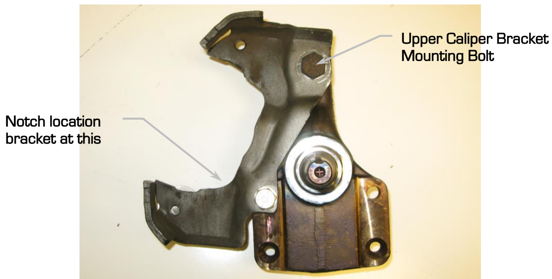
Figure 3 - Notching Stock Caliper Bracket
