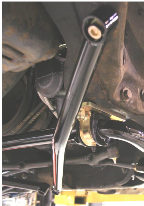
Figure 2 - Completed Installation
