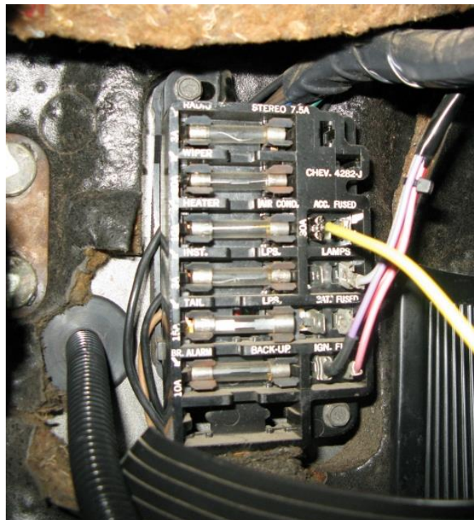
Figure 17 - Connect Power Wire
