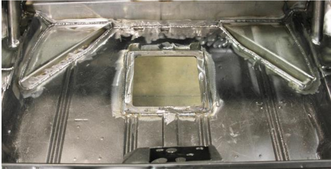
Figure 2 - Mini-Tub Trunk Closeouts on 1969 Camaro
