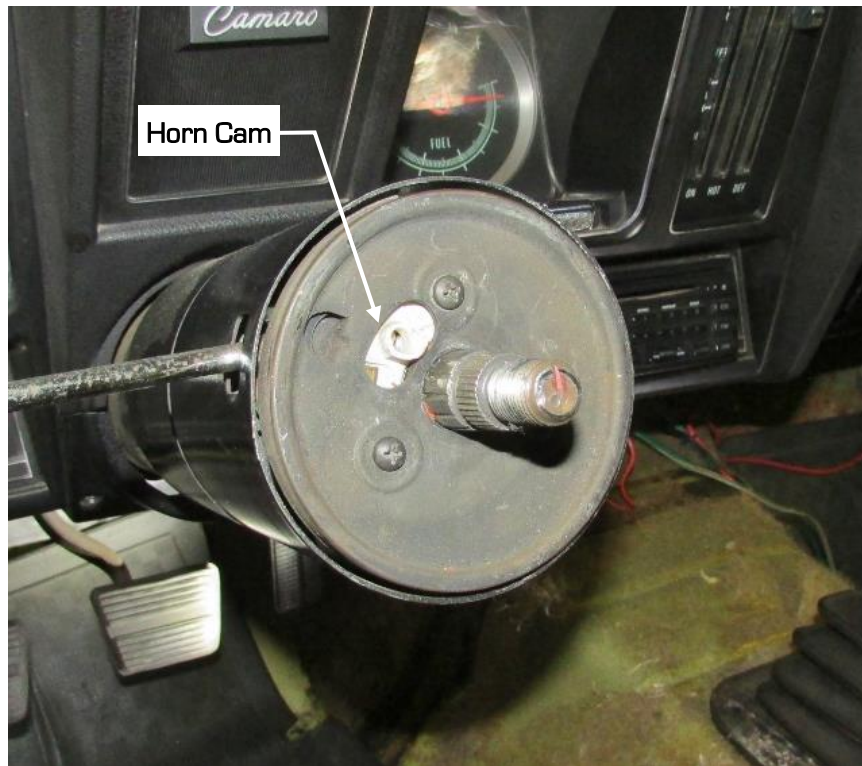
Figure 4 - Locate Horn Cam
