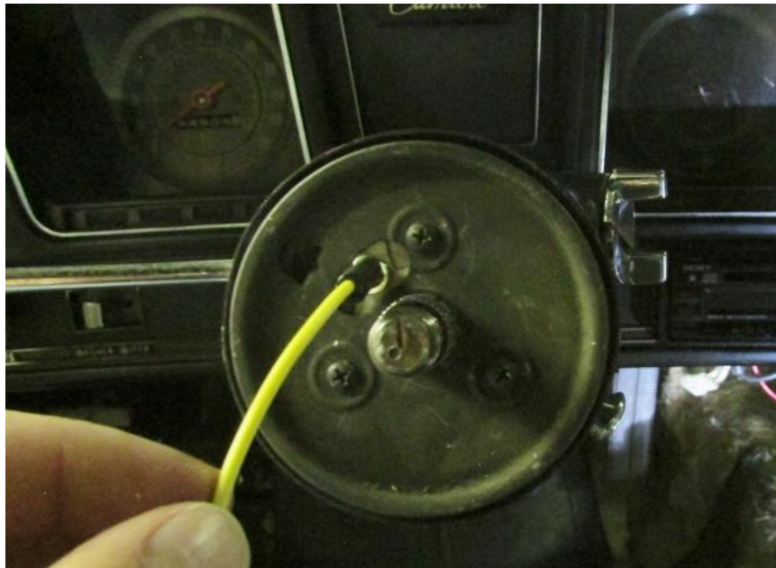
Figure 5 - Install Horn Wire
