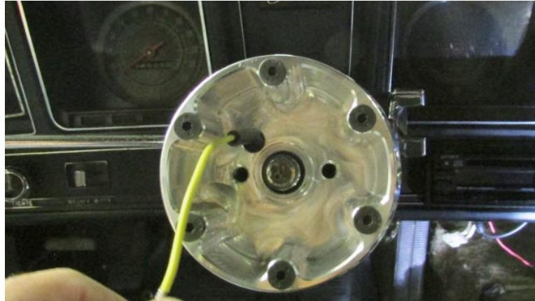
Figure 6 - Install Steering Wheel Adapter
