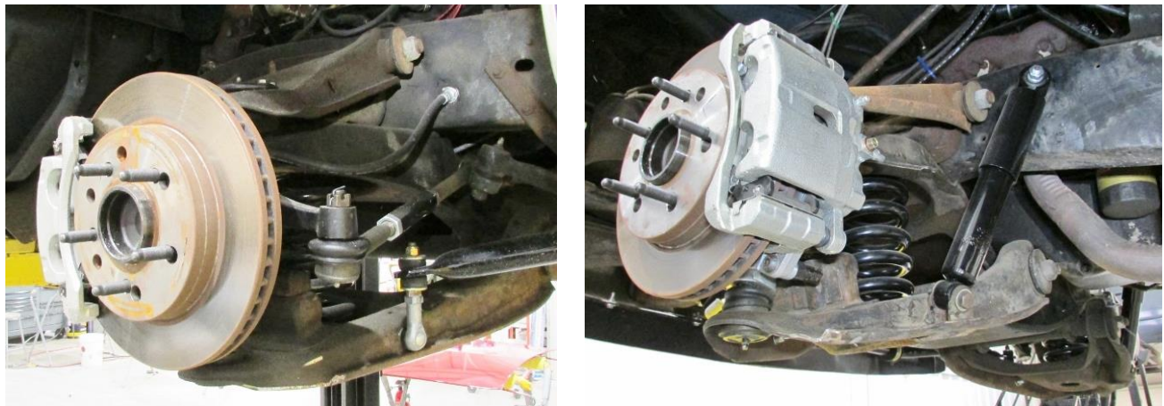
Figure 13 - Speed Kit 2 with DSE Rotor Kit
