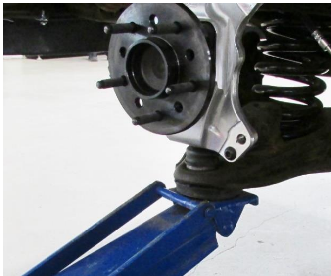
Figure 8 - Install Upright to Upper Ball Joint
