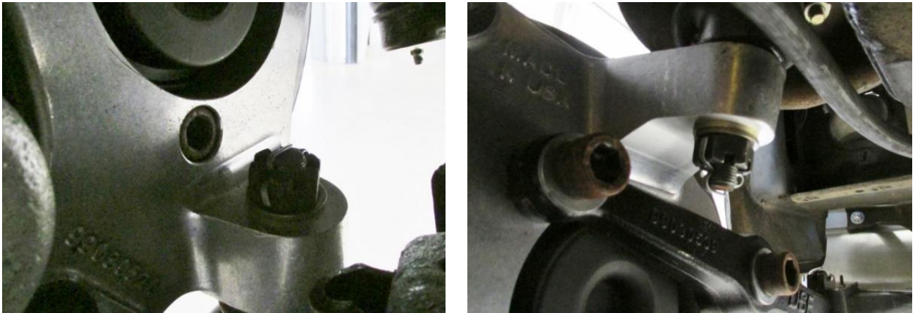
Figure 9 – Install Ball Joint Castle Nuts and Cotter Pins
