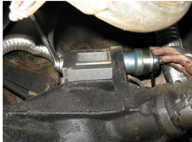
Figure 2 - Bushing Installation
