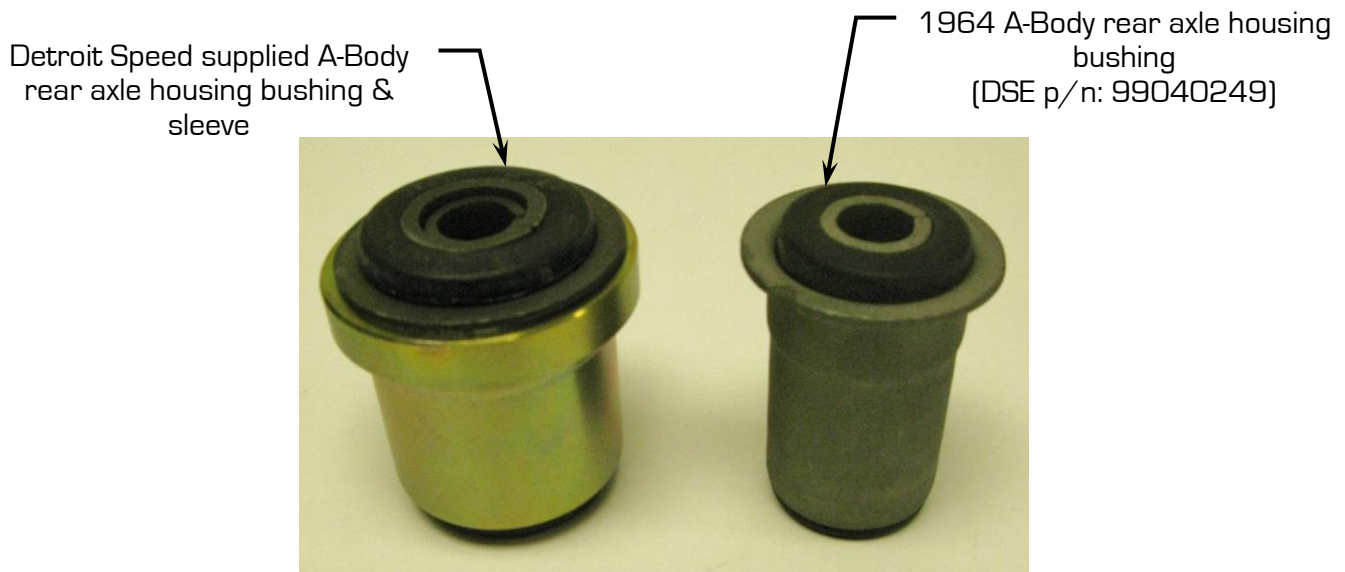
Figure 4 - Rear Axle Bushings
