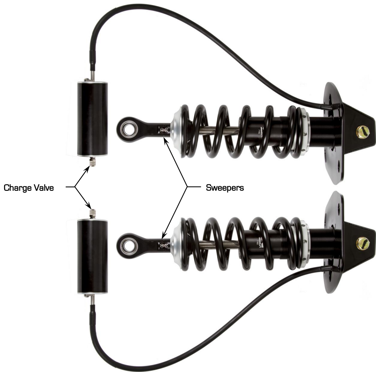
Detroit Speed Double Adjustable Shock with remote canister
