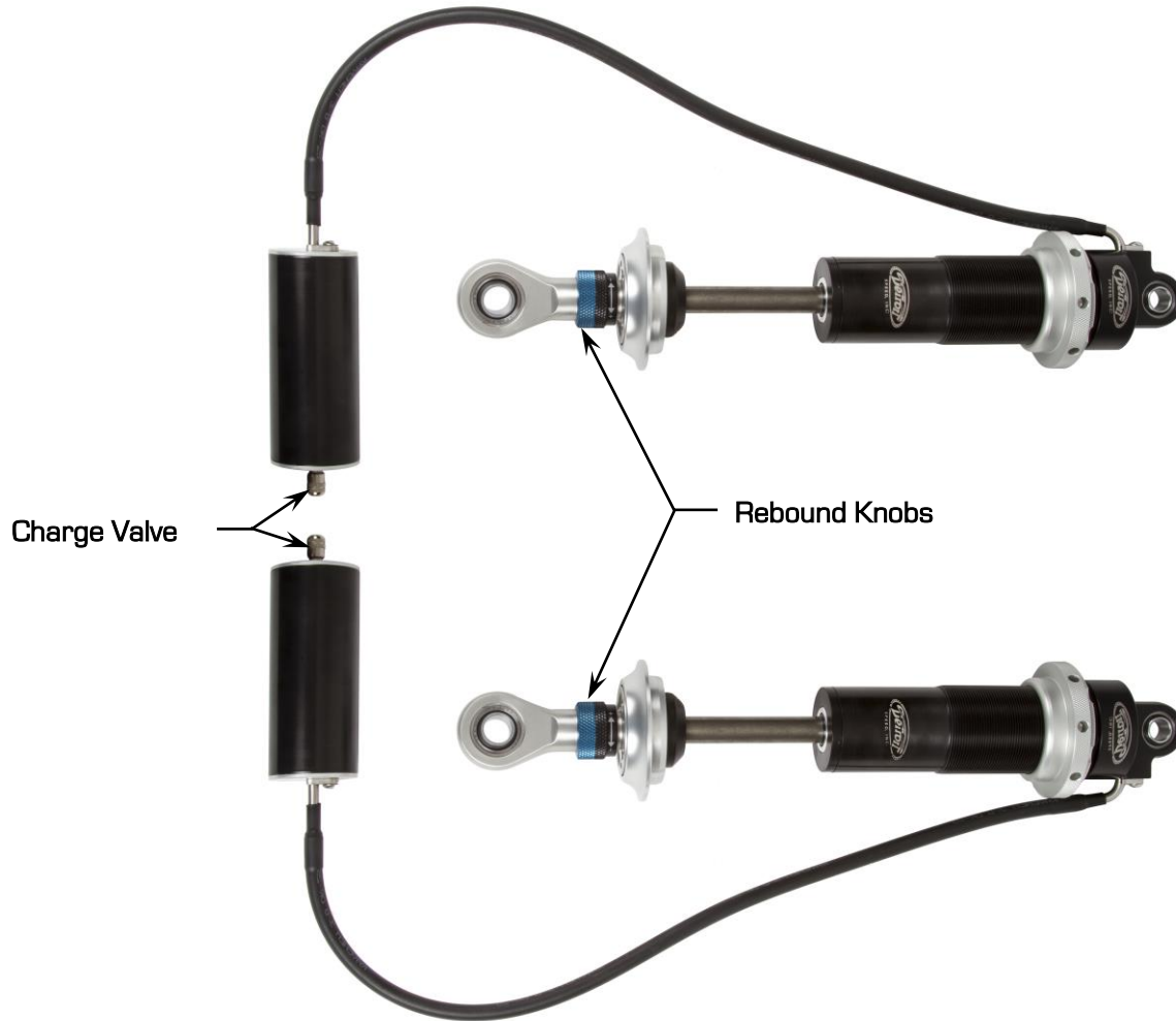
Detroit Speed Single Adjustable Shock w/remote canister
