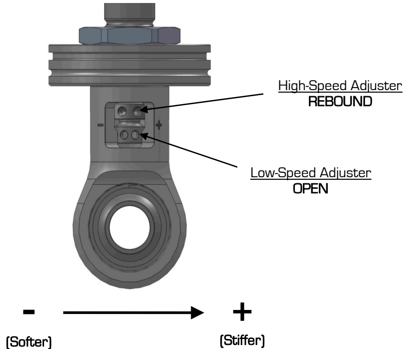
Figure 15b – Detroit Speed Recommended Settings
