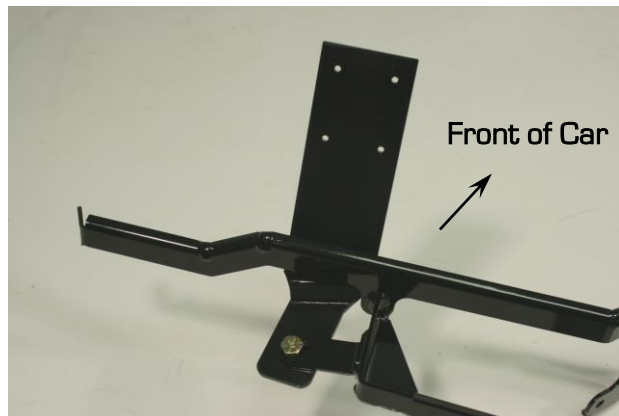
Figure 1 - Plenum Bracket Attached to Gen IV Magnum Mounting Bracket
