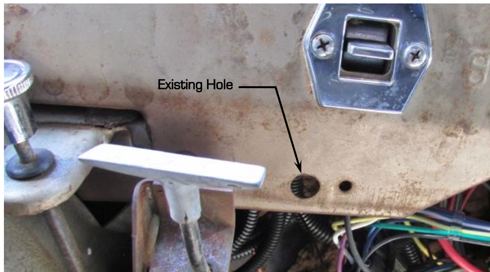
Figure 13 - Control Module Mounting Hole
