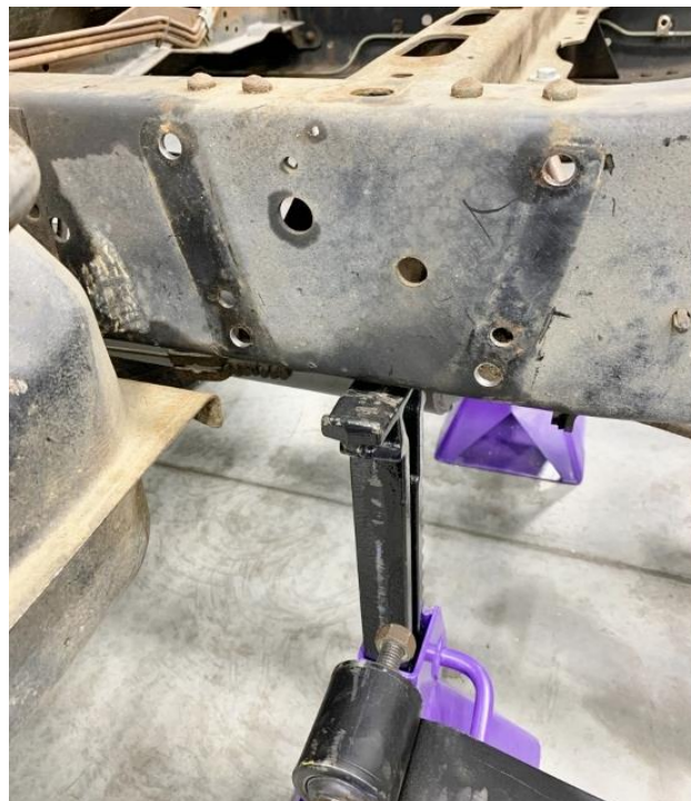
Figure 2 - Drill Out Frame Holes
