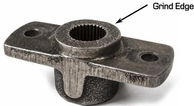
Figure 3 - Modify Coupler
