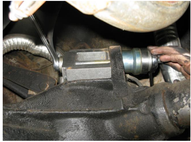
Figure 2 - Bushing Installation
